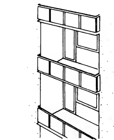
⑤ Inset balconies (loggia)
